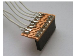
Figure 2.3 Using Veroboard
