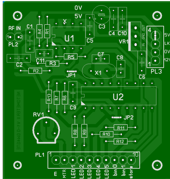
Figure 2.1. PCB Layout
