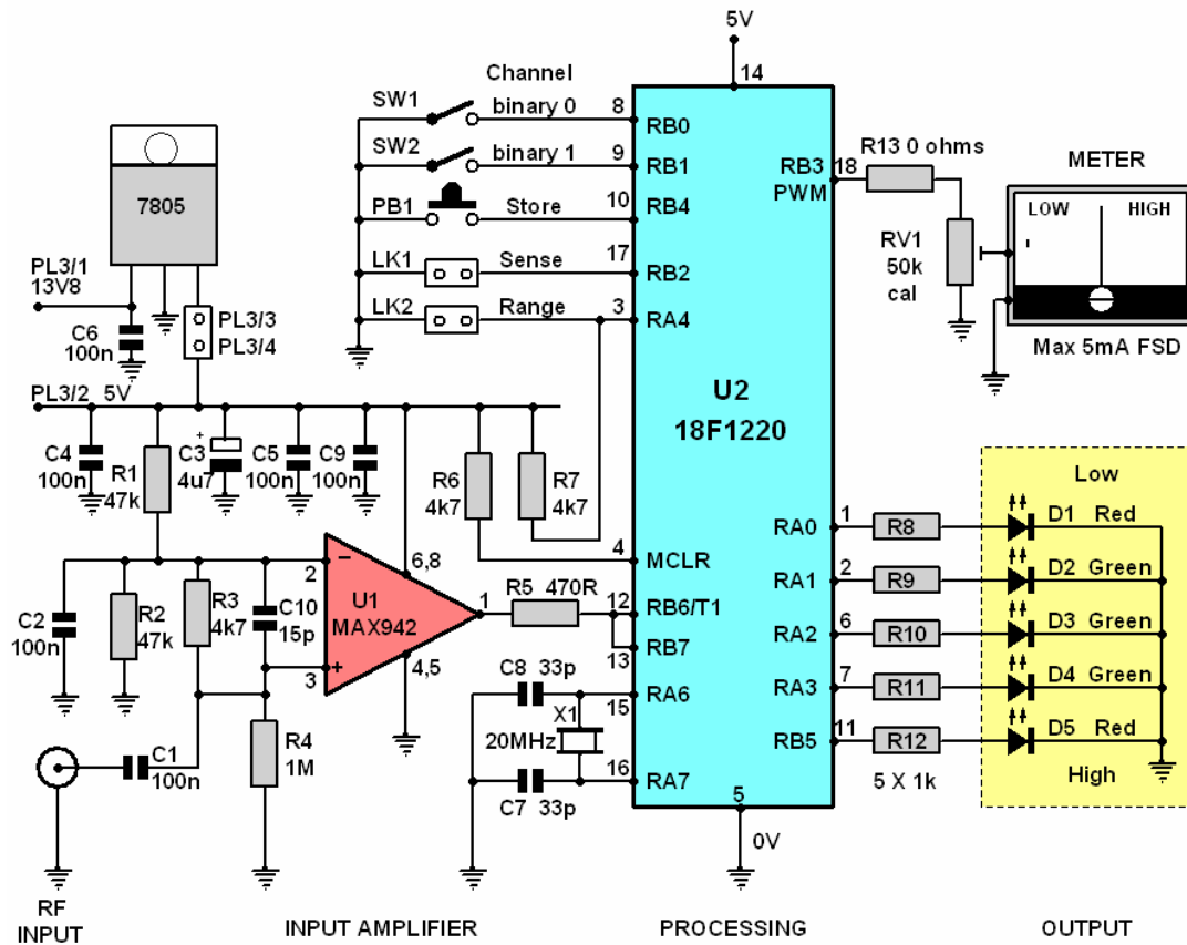
Figure 1.1 Circuit Diagram
